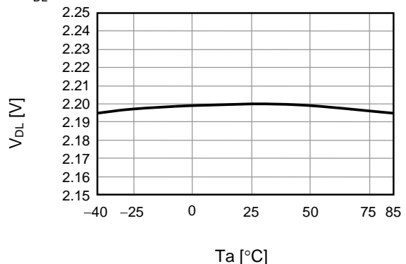
4. V_{DL} - T_a
