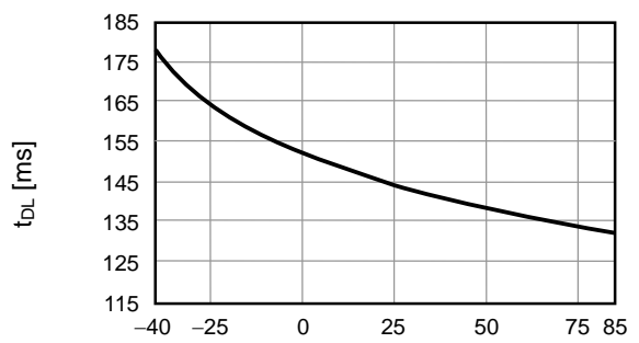
6. t_{DL} - T_a
