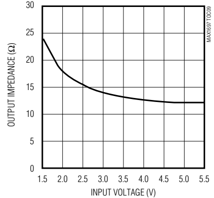
MAX1697R/S/T/U OUTPUT IMPEDANCE vs. INPUT VOLTAGE
