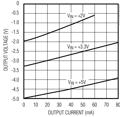
MAX1697S OUTPUT VOLTAGE vs. OUTPUT CURRENT
