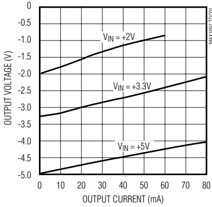
MAX1697R OUTPUT VOLTAGE vs. OUTPUT CURRENT
