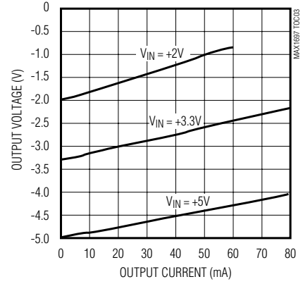
MAX1697T OUTPUT VOLTAGE vs. OUTPUT CURRENT
