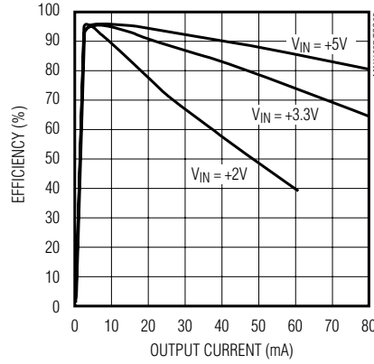
MAX1697U EFFICIENCY vs. OUTPUT CURRENT
