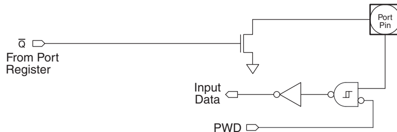
Figure 10-4. Open-Drain Output
