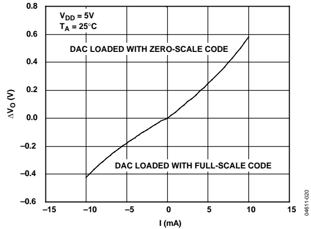
Figure 20. Sink and Source Capability
