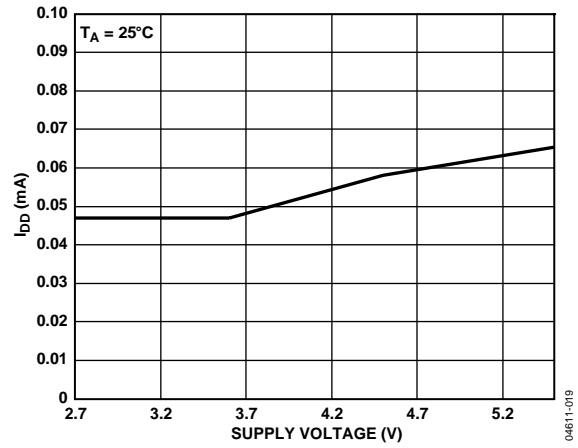
Figure 19. Supply Current vs. Supply Voltage at 25°C
