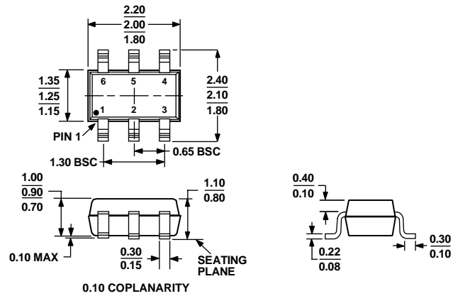
Figure 45. 6-Lead Thin Shrink Small Outline Transistor Package [SC70] (KS-6) Dimensions shown in millimeters
