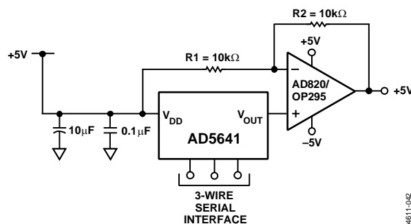
Figure 43. Bipolar Operation with the AD5641
