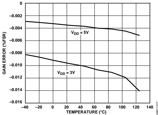
Figure 17. Gain Error vs. Temperature (3 V/5 V)
