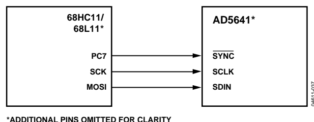
Figure 38. AD5641 to 68HC11/68L11 Interface
