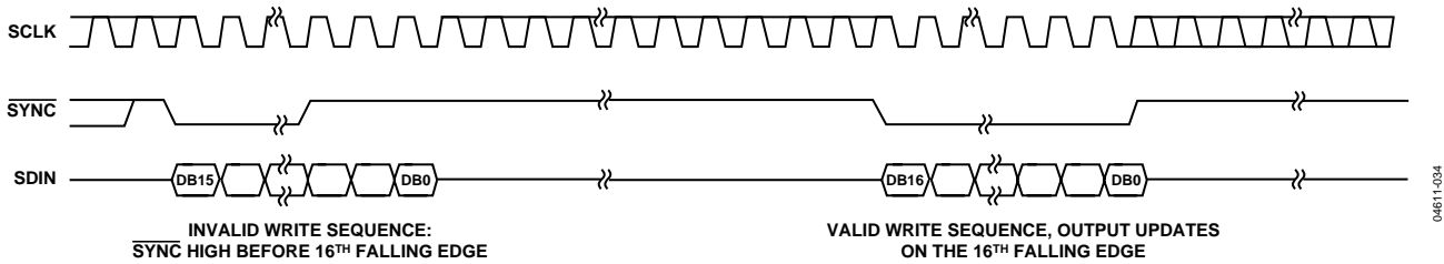
Figure 35. \overline{SYNC} Interrupt Facility
