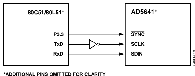
Figure 40. AD5641 to 80C51/80L51 Interface
