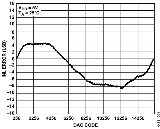
Figure 4. Typical INL
