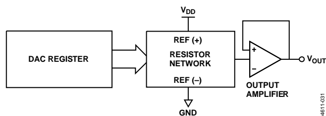
Figure 32. DAC Architecture
