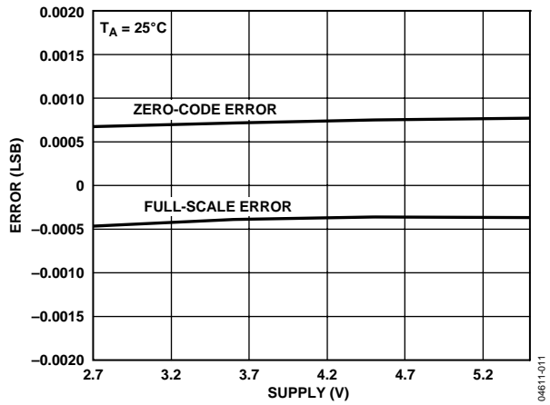
Figure 11. Zero-Code/Full-Scale Error vs. Supply at 25°C
