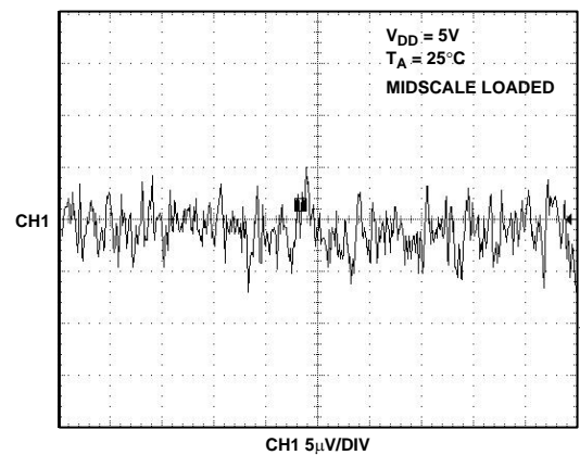
Figure 27. 1/f Noise, 0.1 Hz to 10 Hz Bandwidth
