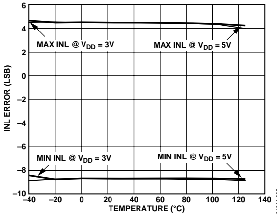
Figure 5. INL Error vs. Temperature (3 V/5 V Supply)
