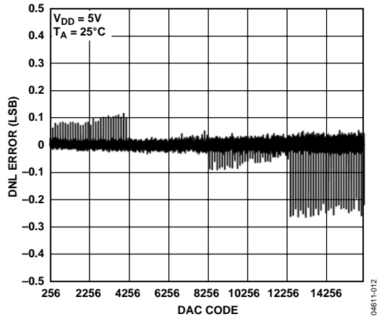
Figure 12. Typical DNL
