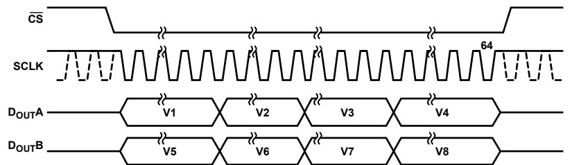
Figure 46. AD7606 Serial Interface with Two D_{OUT} Lines
